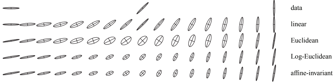
Fig. 3. \lambda = 0, \mu = 10^3 . Geodesic-like regression. The Euclidean and Log-Euclidean metric solutions are accurate and quick to compute. The affine-invariant metric solution is noticeably slower to compute and its precision depends on the stopping criterion of Algorithm 2.
